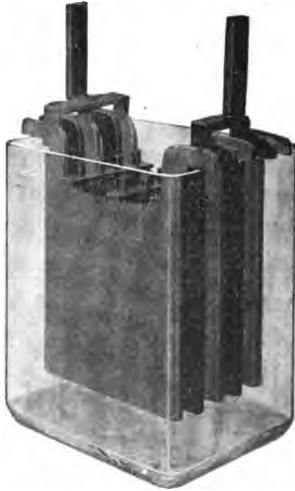
FIG. 448.—A Typical Storage Cell Enclosed in a Glass Jar. This cell represents one of the best-known makes of the Planté genus. With five plates, as shown, such a cell has a capacity of 80 ampere-hours, at 8 hours' discharge; of 70 ampere-hours, at 5 hours' discharge; of 60 ampere-hours, at 3 hours' discharge; with a discharge rate of 10 amperes in 8 hours; of 14 amperes in 5 hours, and of 20 amperes in 3 hours. The total outside dimensions of this cell are 5\frac{1}{4} \times 9\frac{1}{4} \times 11\frac{1}{4} inches; dimensions of each plate's active surface, 7\frac{3}{4} \times 7\frac{3}{4} inches.
